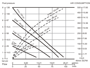
(* 2 bar test with a pump fitted with PTFE (Teflon®) diaphragms. — Outlet pressure — Air consumption
